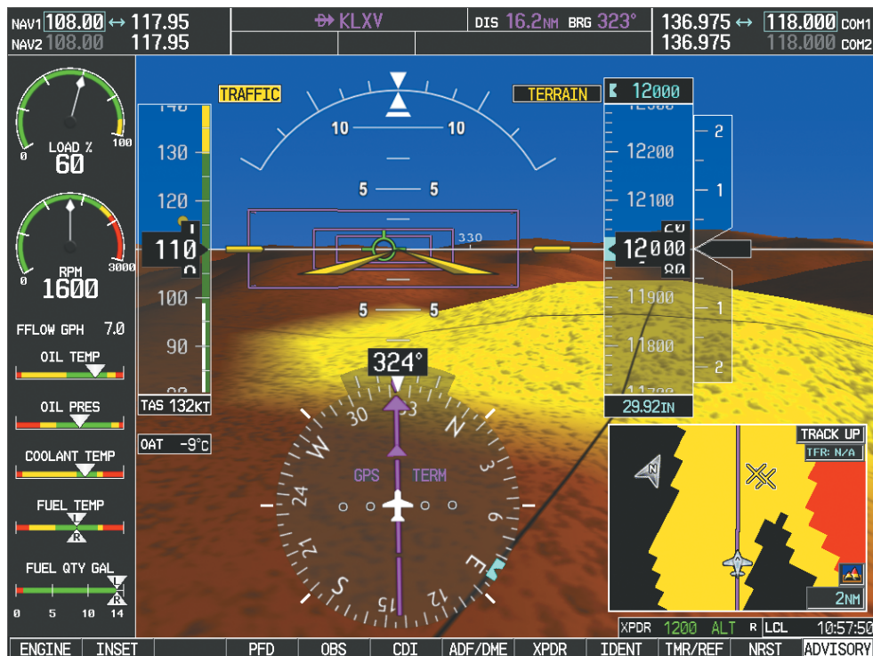
Figure 8-88 SVS Reversionary Mode
