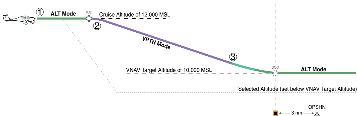
Figure 7-35 VPTH Descent
