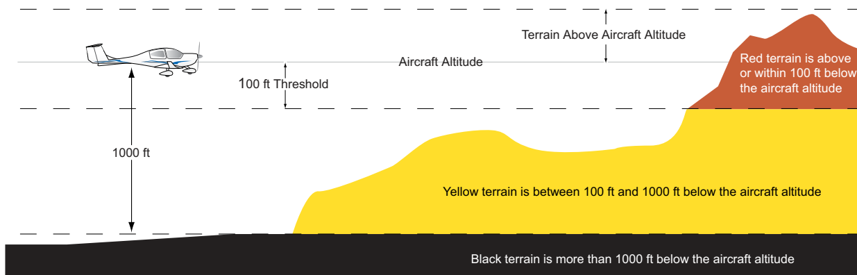
Figure F-1 Terrain Altitude/Color Correlation
