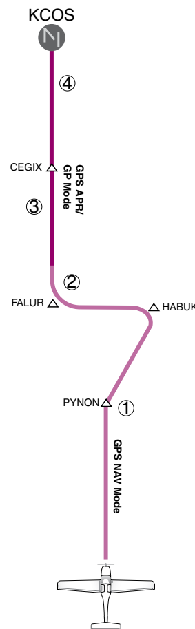
Figure 7-38 LPV Approach to KCOS
