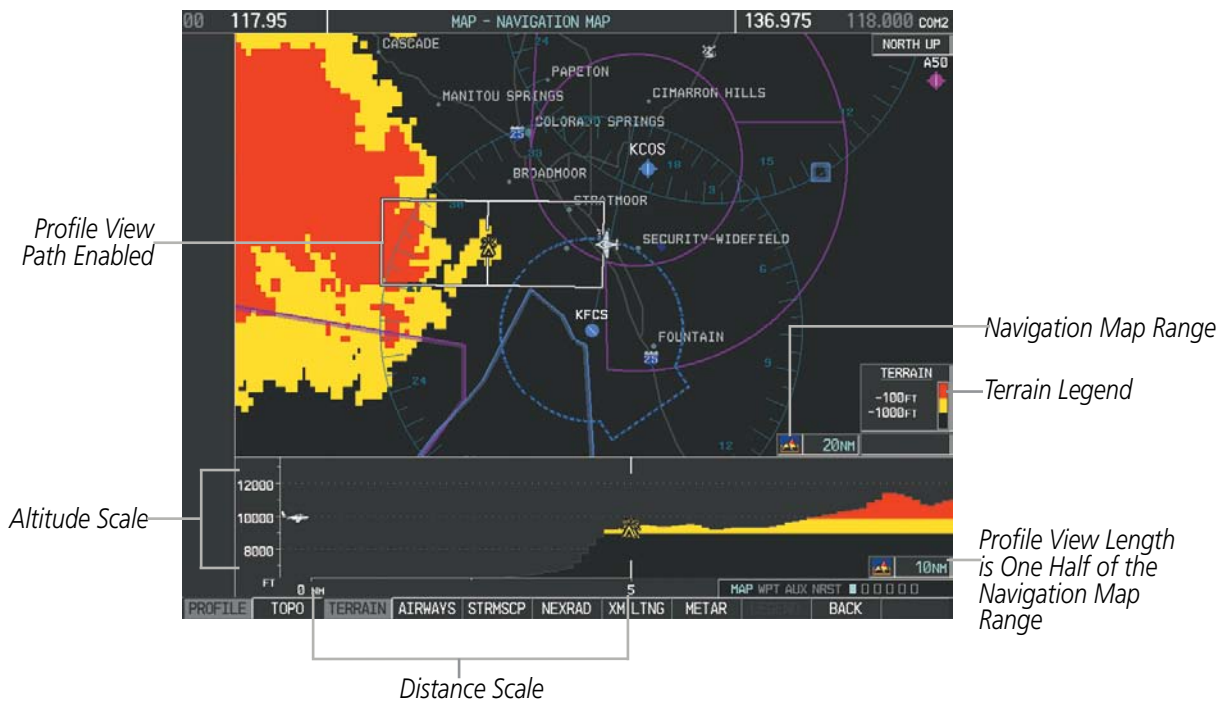
Figure 6-68 Profile View on Navigation Map with Terrain Display Enabled
