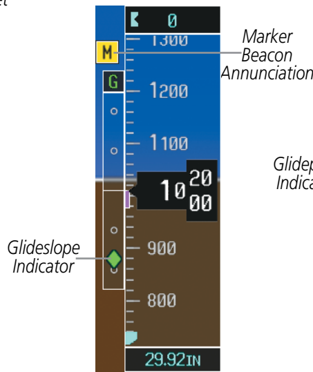
Figure 2-12 Glideslope Indicator
