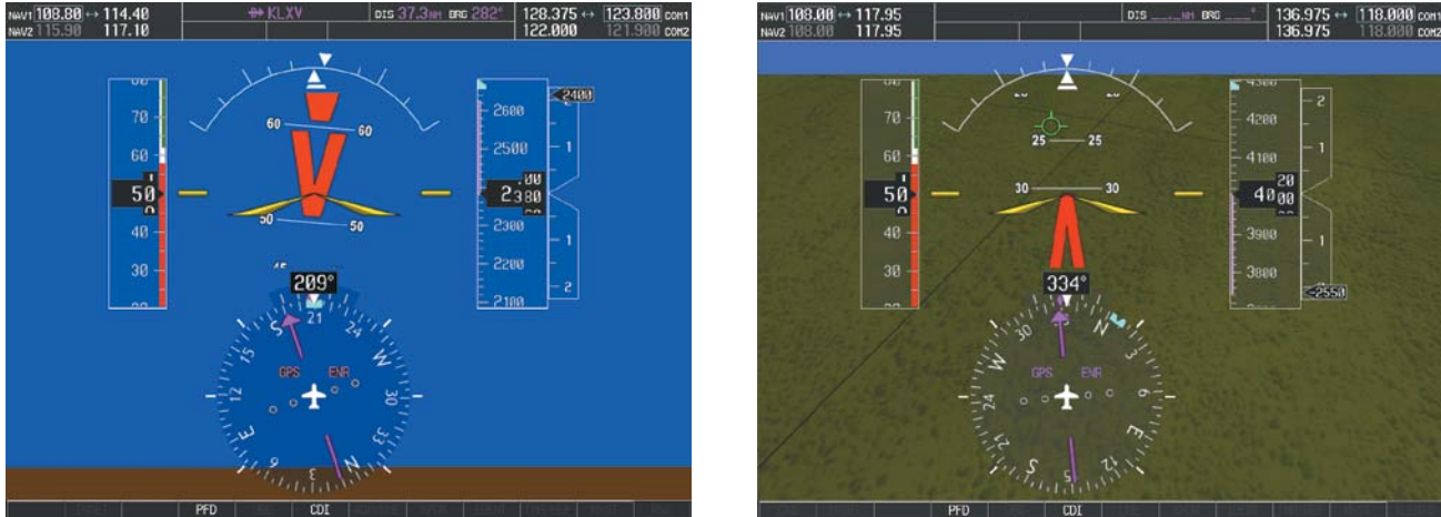
Figure 8-89 Unusual Attitude Display
