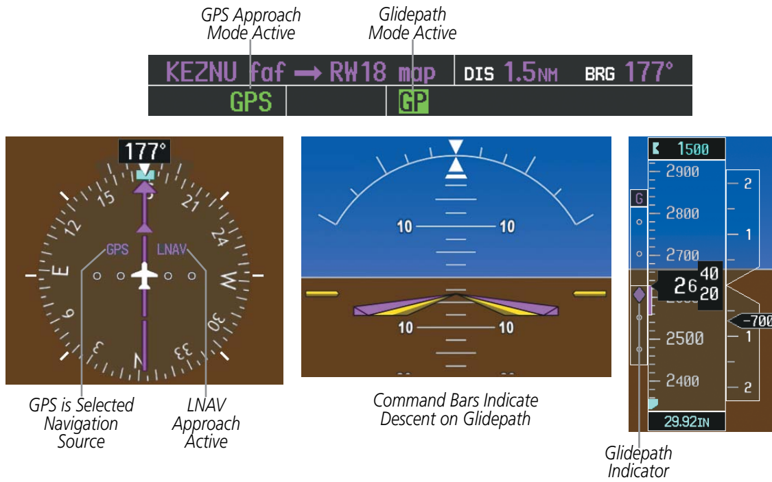
Figure 7-16 Glidepath Mode
