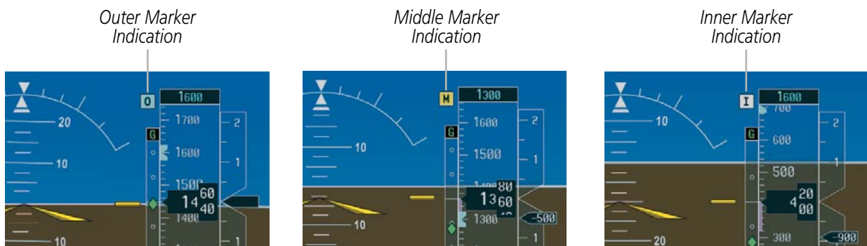
Figure 4-27 Marker Beacon Annunciations on the PFD
