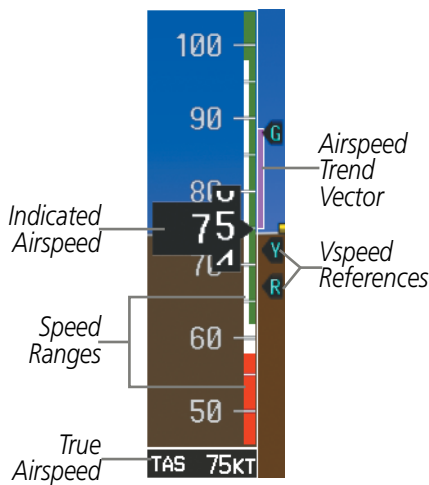
Figure 2-3 Airspeed Indicator
