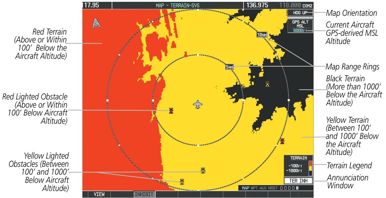
Figure 6-77 Terrain-SVS Page (360 View)
