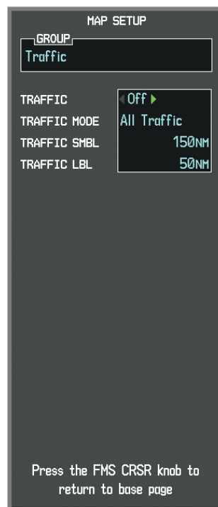
Figure 6-86 Navigation Map Page Setup Menu, Traffic Group
