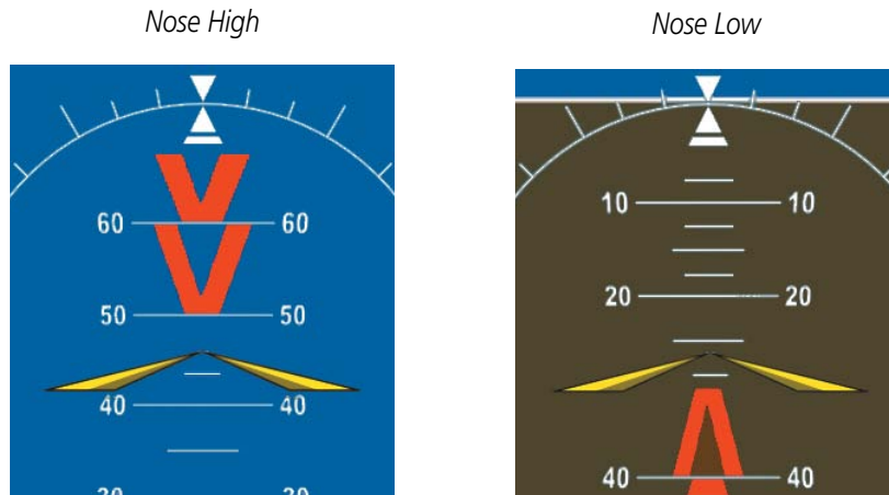
Figure 2-43 Pitch Attitude Warnings
