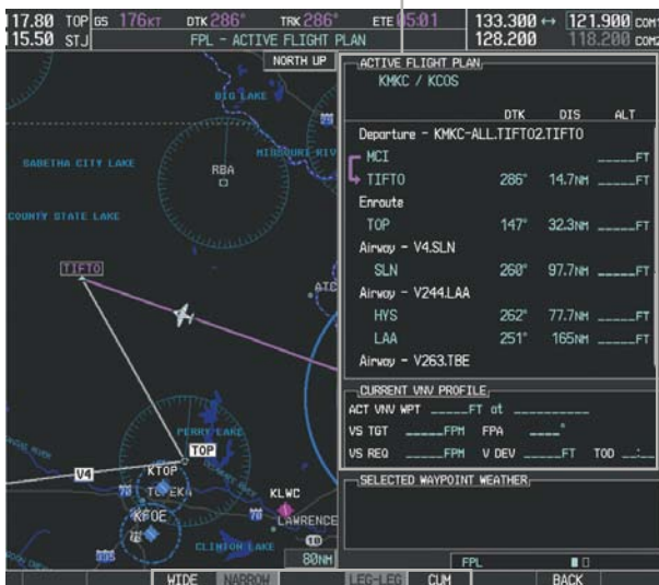
Flight Plan View Softkeys WIDE, NARROW, LEG-LEG, CUM
