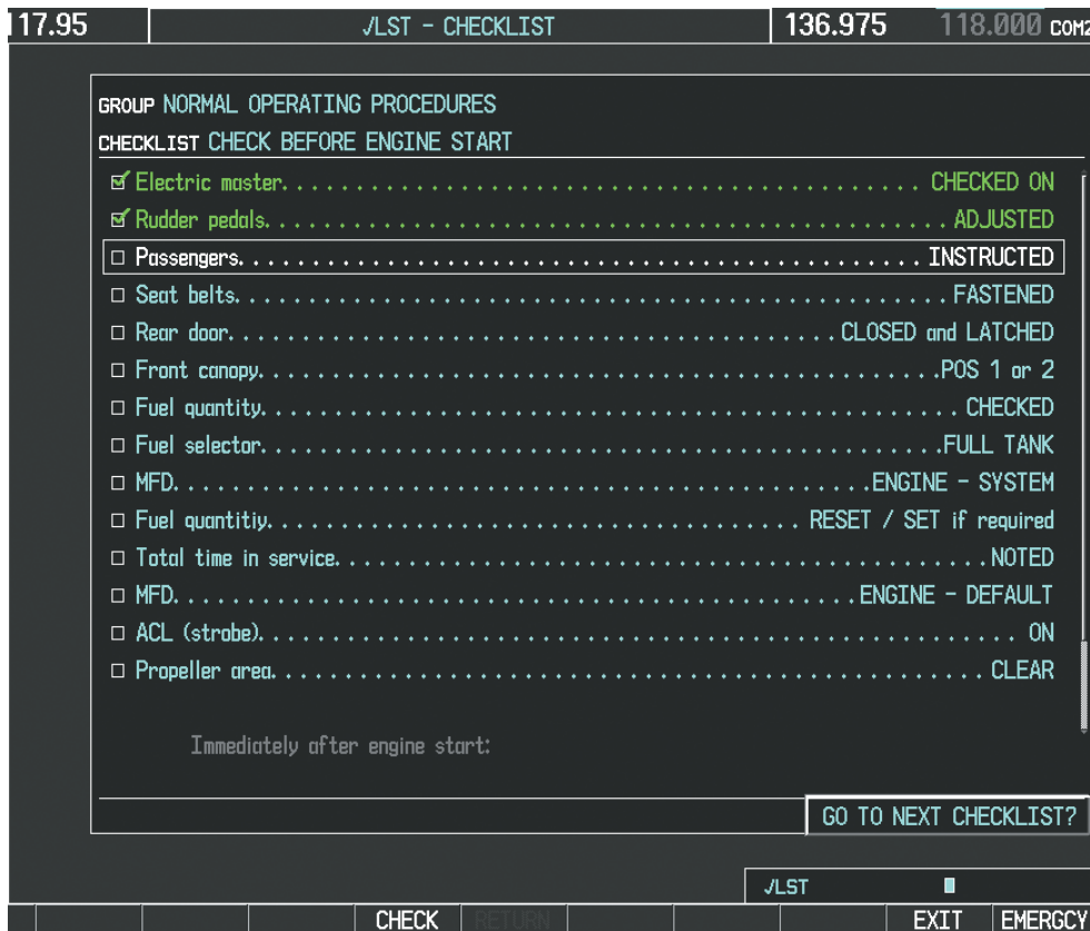
Figure 8-81 Sample Checklist
