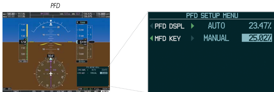
Figure 1-36 PFD Setup Menu
