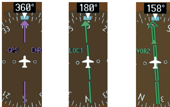
Figure 2-22 Navigation Sources
