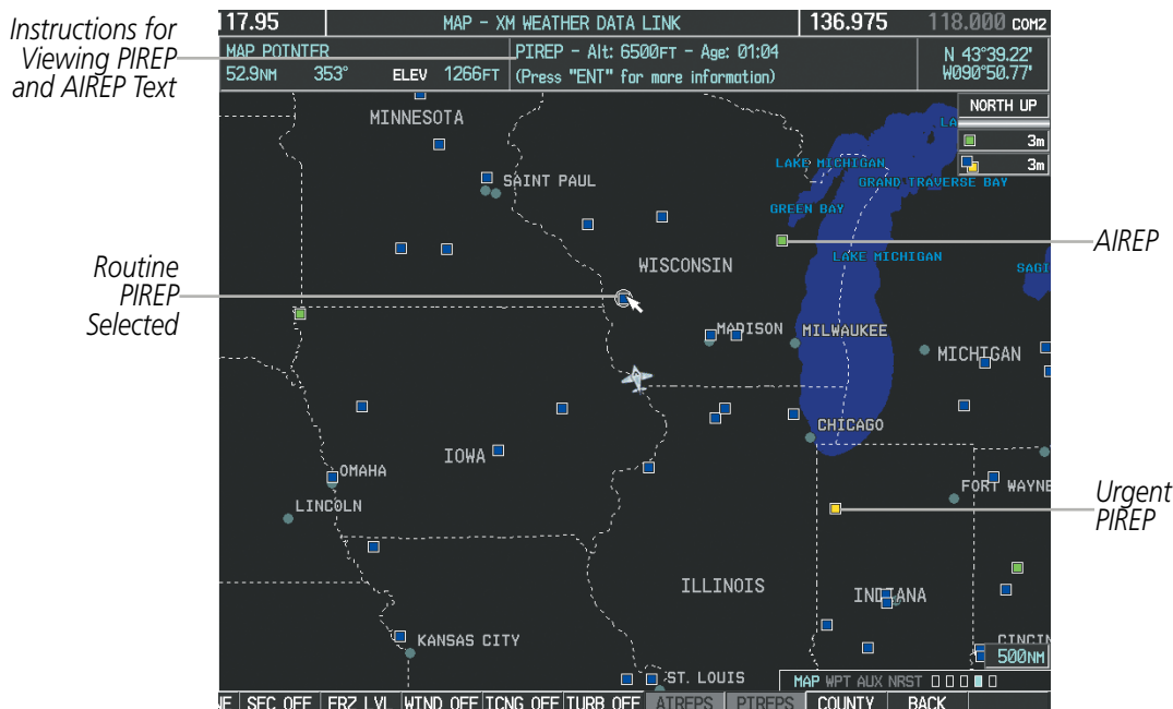
Figure 6-46 AIREPs and PIREPs on the XM Weather Data Link Page
