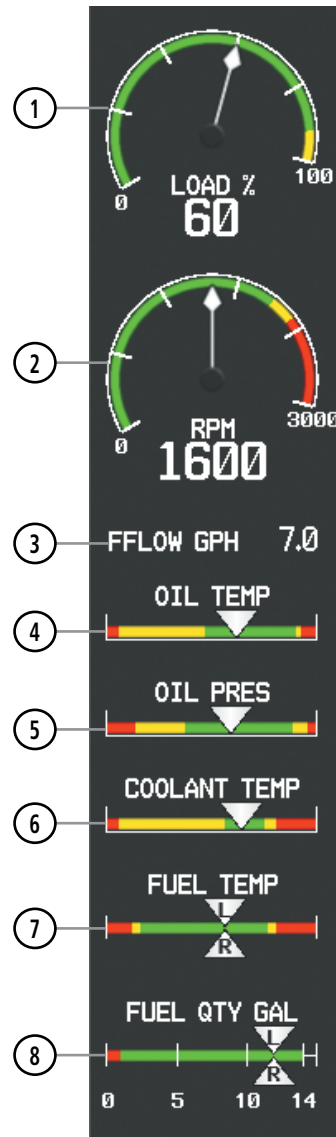
Figure 3-2 Engine Display
