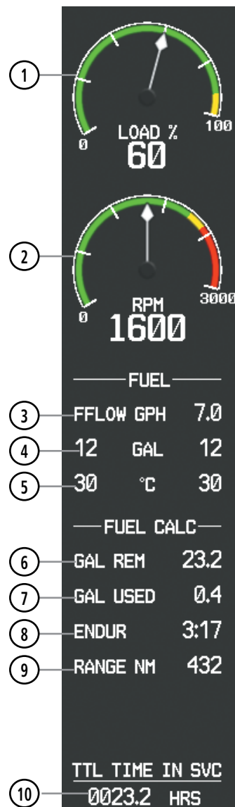
Figure 3-4 Fuel Display
