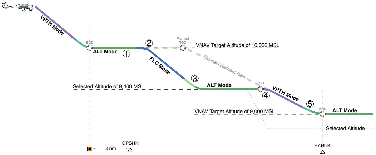
Figure 7-36 Non-path Descent
