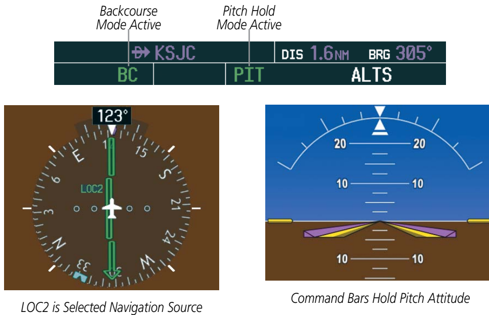
Figure 7-24 Backcourse Mode
