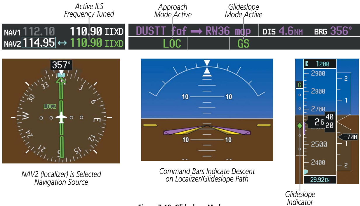
Figure 7-18 Glideslope Mode
