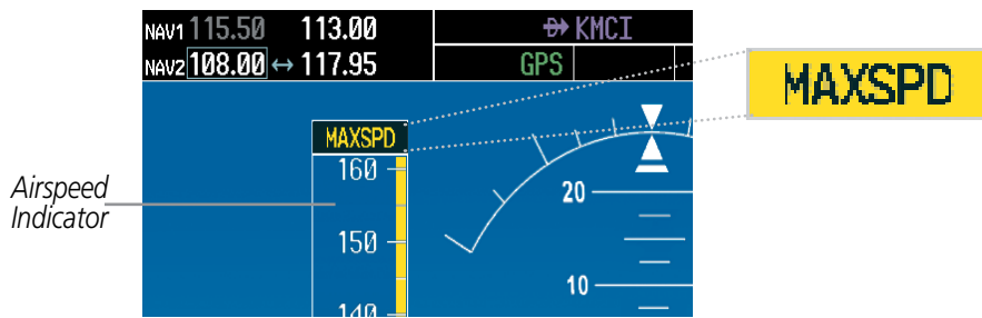
Figure 7-41 Overspeed Annunciation
