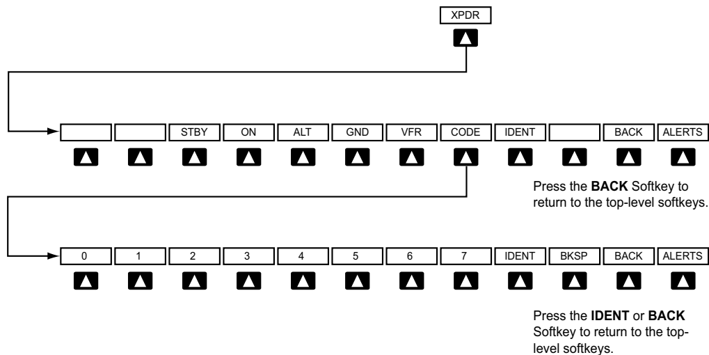
Figure 1-19 XPDR Softkeys
