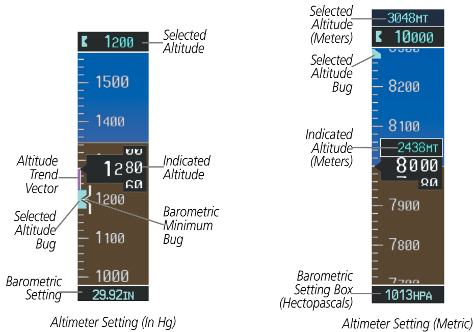
Figure 2-9 Altimeter Settings, In Hg and Metric
