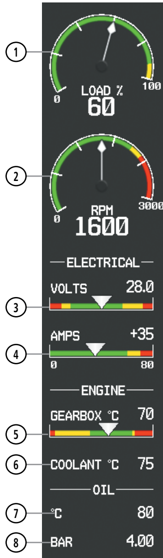
Figure 3-3 System Display
