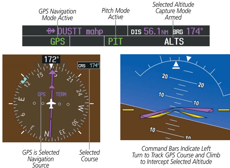
Figure 7-23 Navigation Mode
