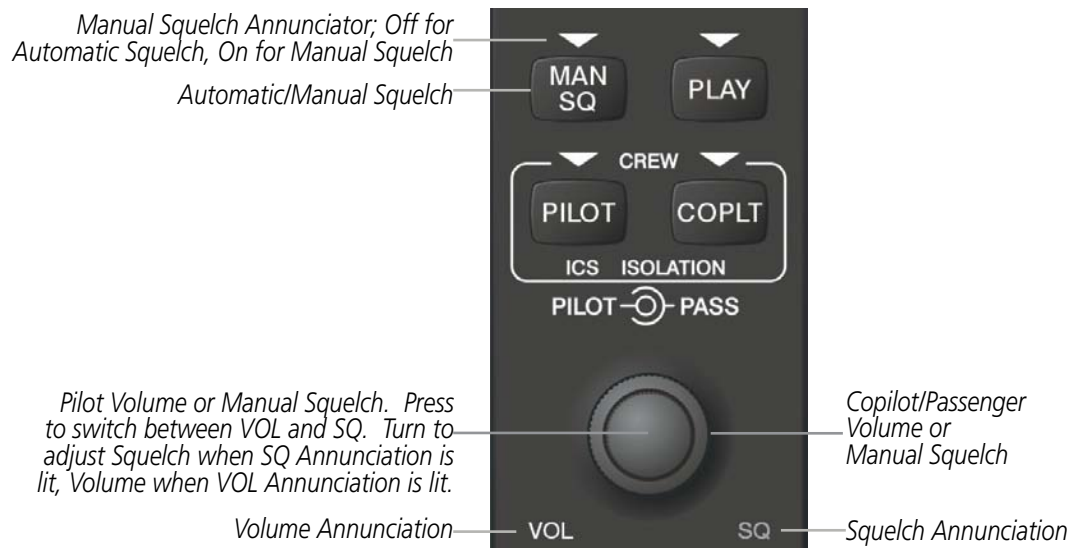
Figure 4-47 Volume/Squelch Control
