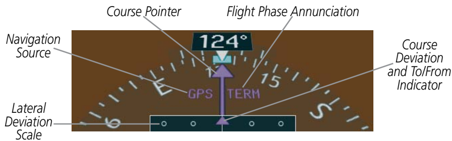
Figure 2-15 Arc HSI
