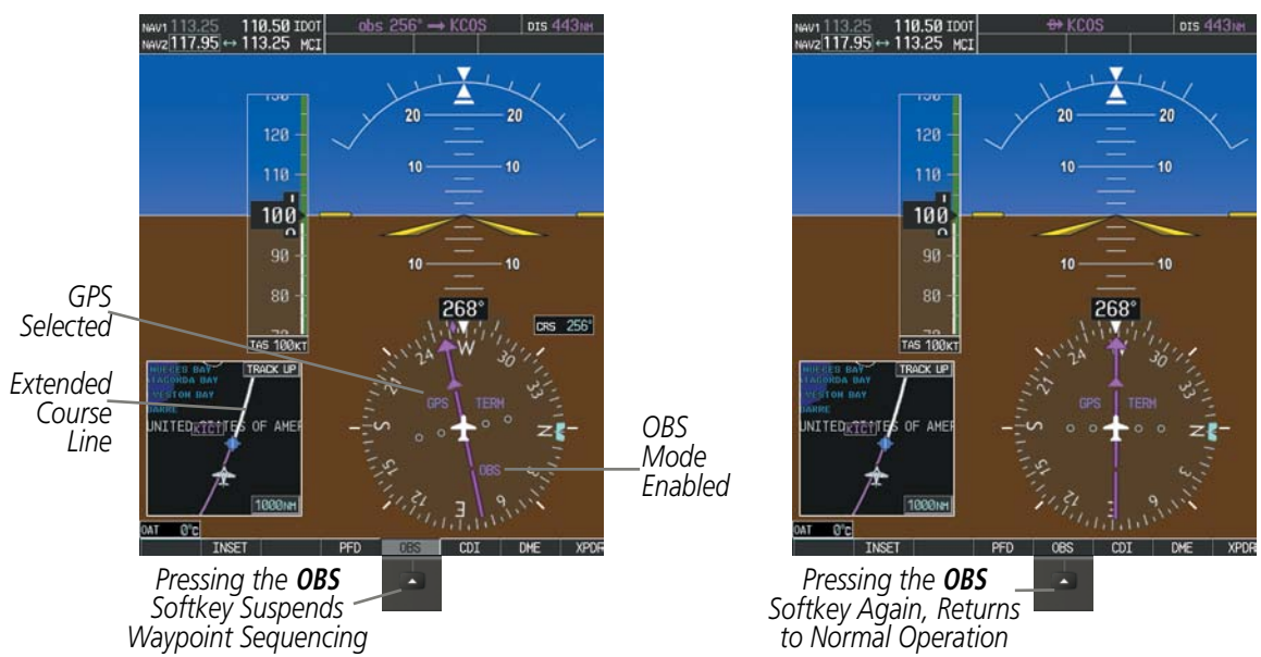
Figure 2-28 Omni-bearing Selector (OBS) Mode
