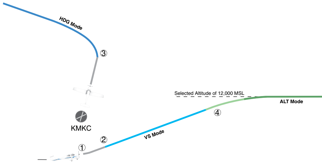
Figure 7-31 Departure
