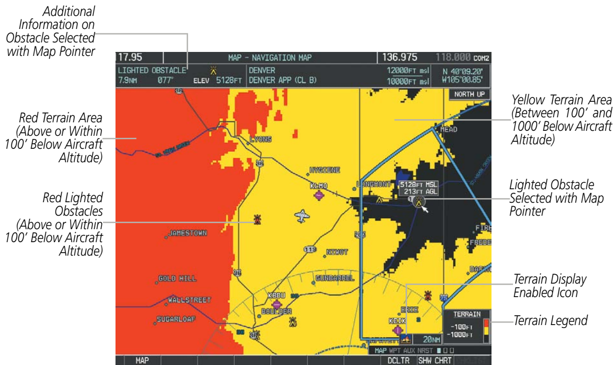
Figure 6-64 Terrain Information on the Navigation Map Page
