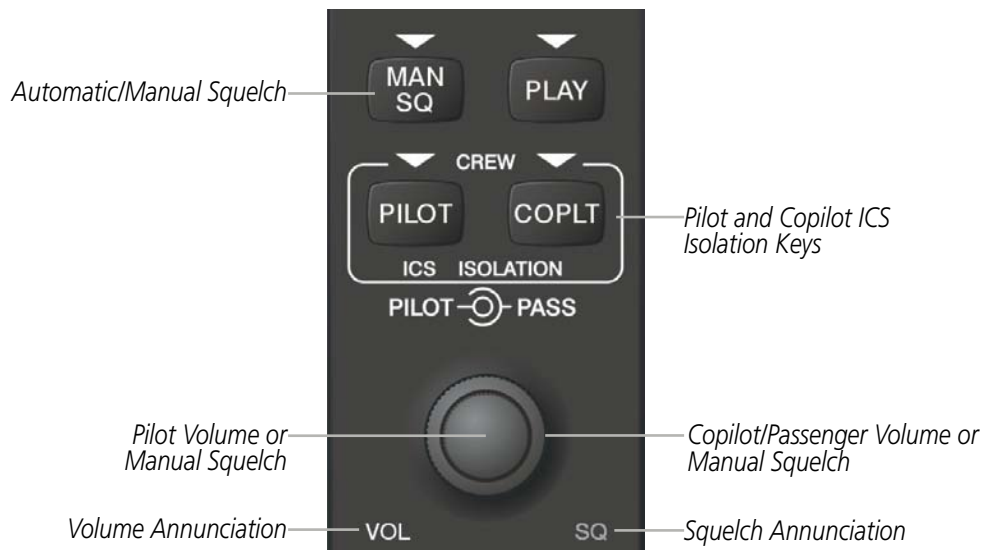
Figure 4-50 Audio Panel Controls
