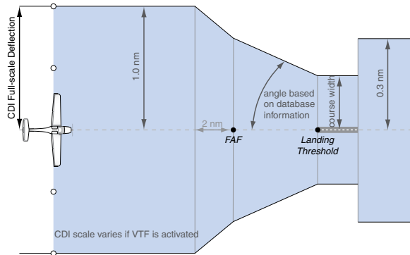
Figure 2-27 Typical LNAV/VNAV and LPV Approach CDI Scaling
