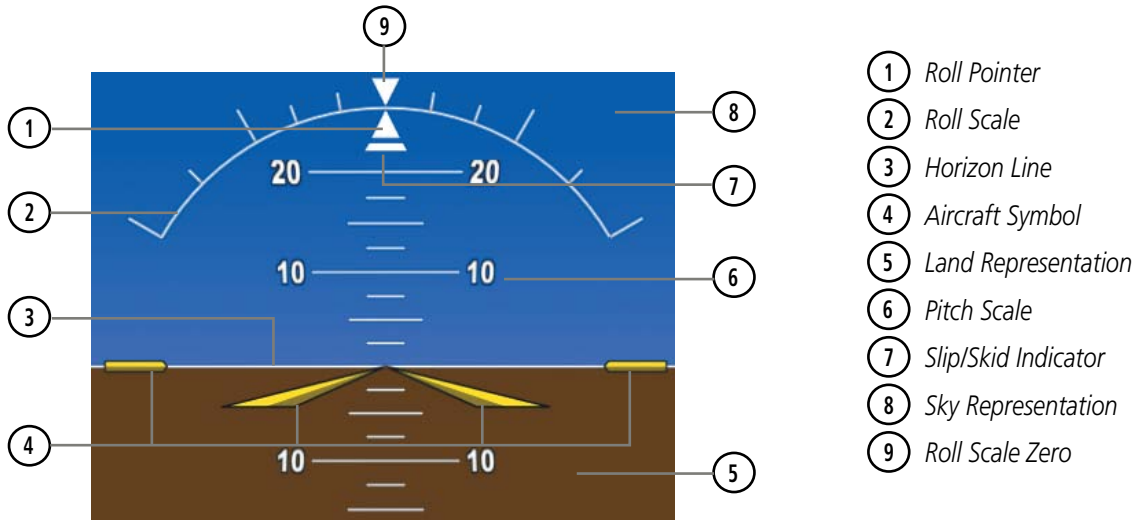
Figure 2-7 Attitude Indicator
