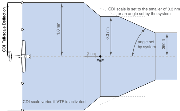
Figure 2-26 Typical LNAV and LNAV+V Approach CDI Scaling
