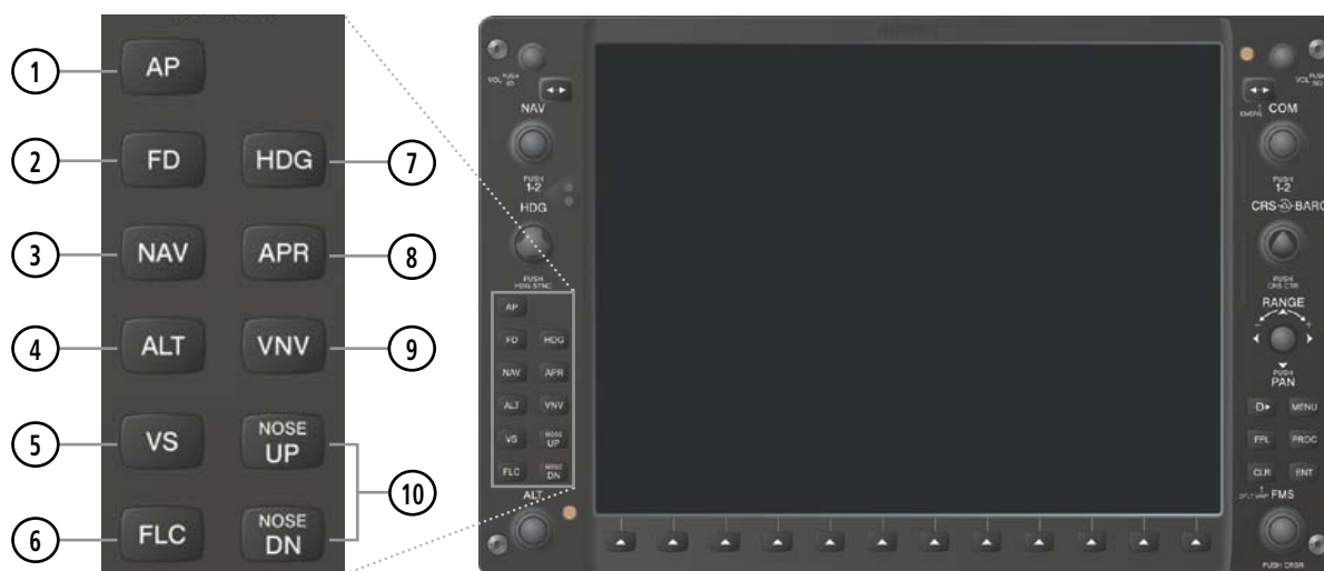
Figure 7-1 Dedicated MFD AFCS Controls (GDU 1044)
