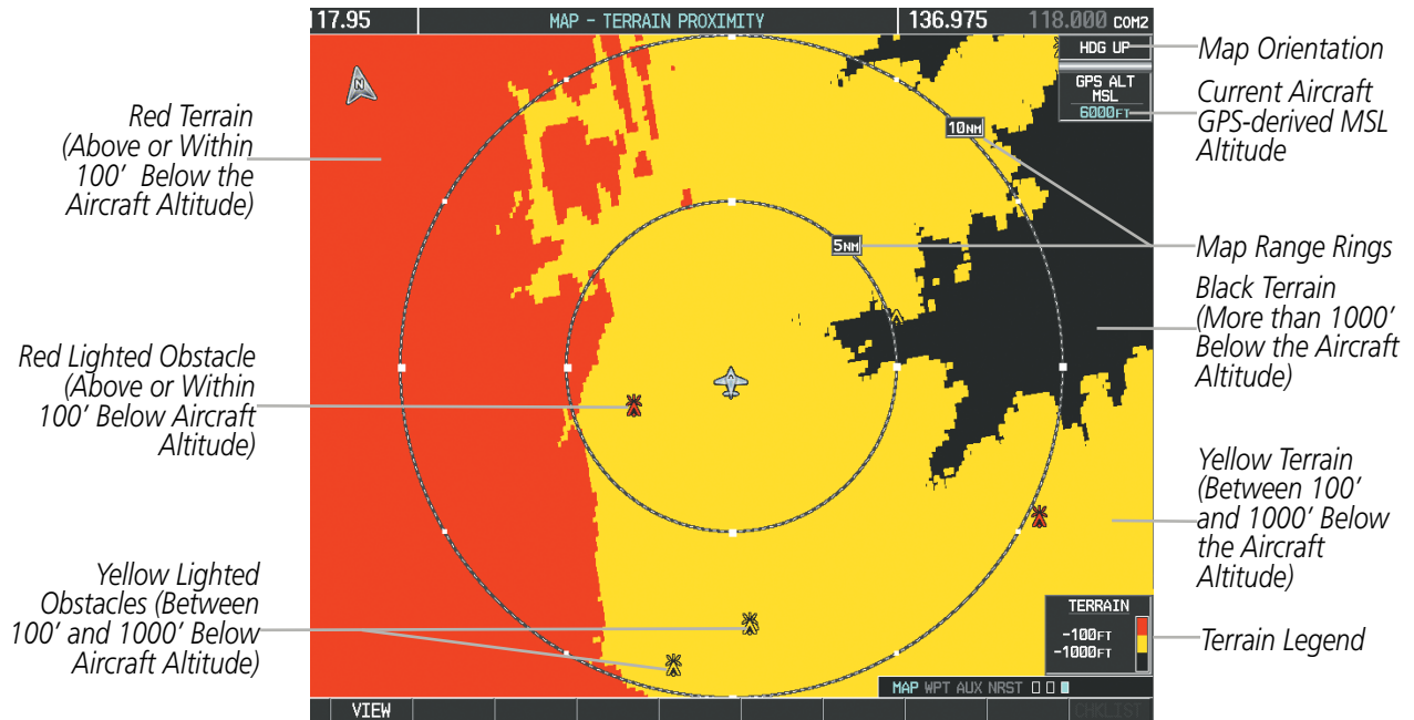
Figure 6-65 Terrain Proximity Page
