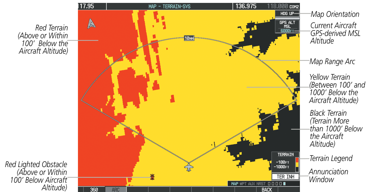
Figure 6-78 Terrain-SVS Page (ARC View)
